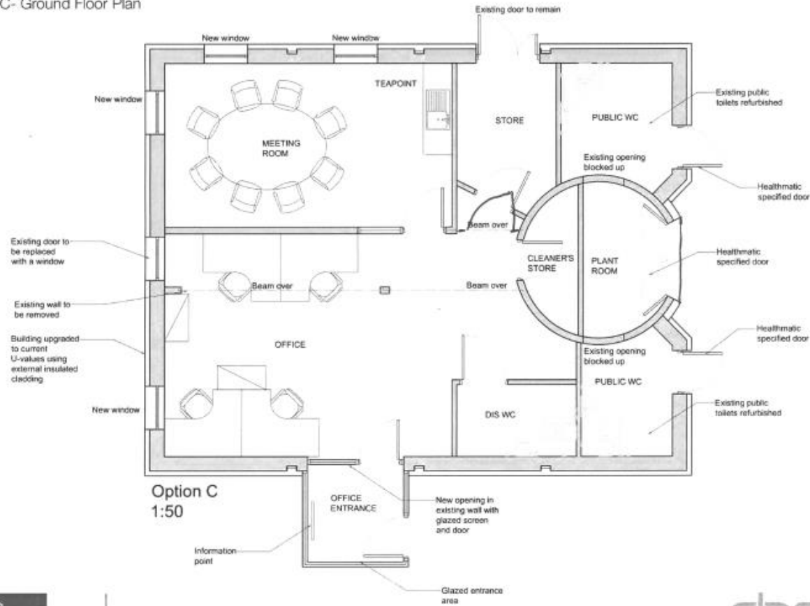
6.2 Option C- Ground Floor Plan
